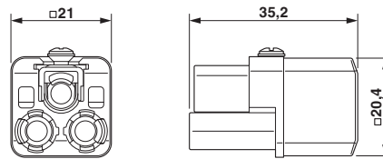
Dimensional drawing
